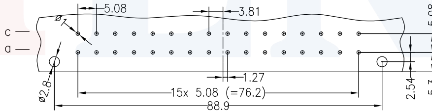
PCB LAYOUT (RECOMMENDED)
